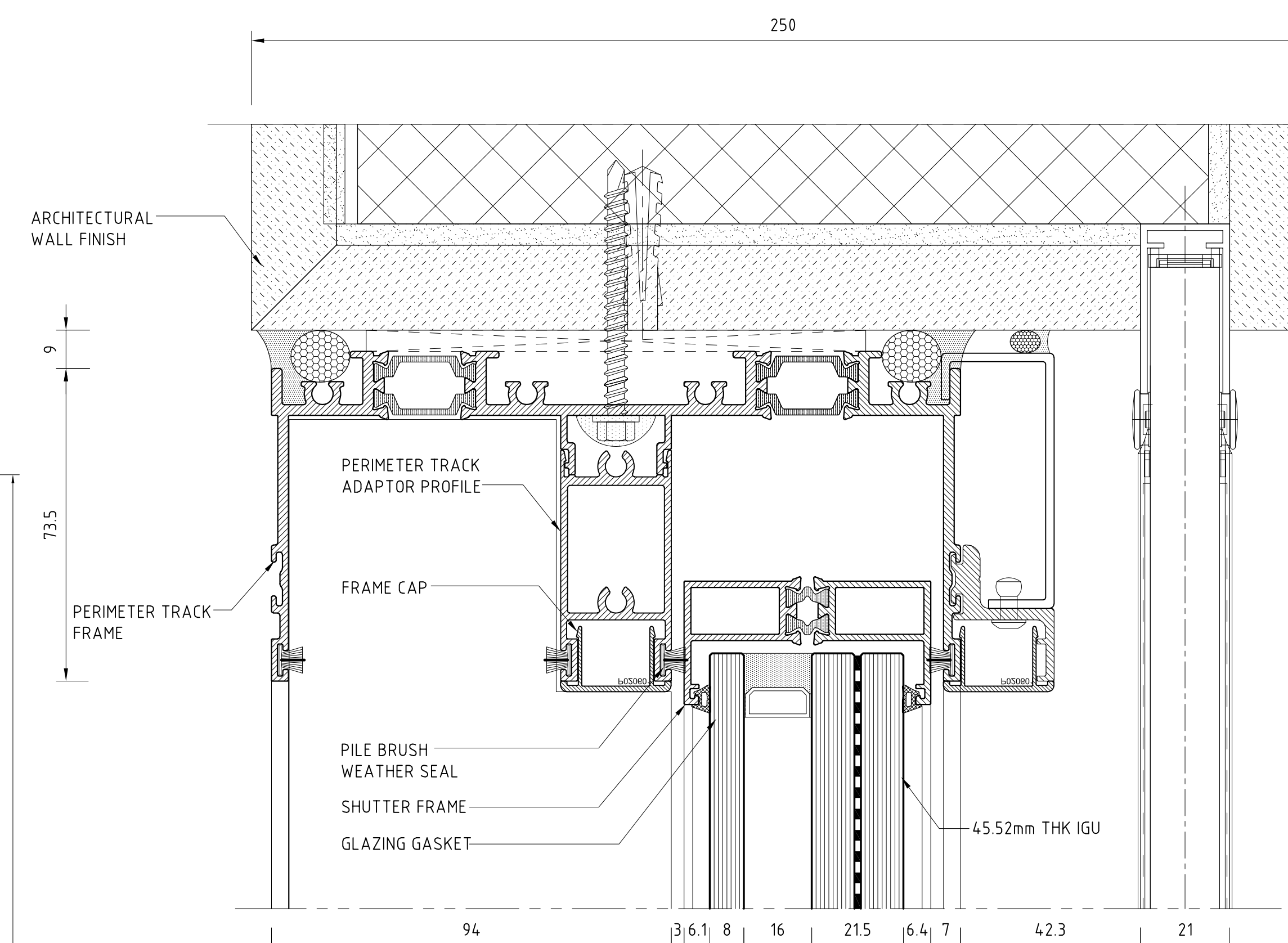
HEAD RAIL DETAIL
