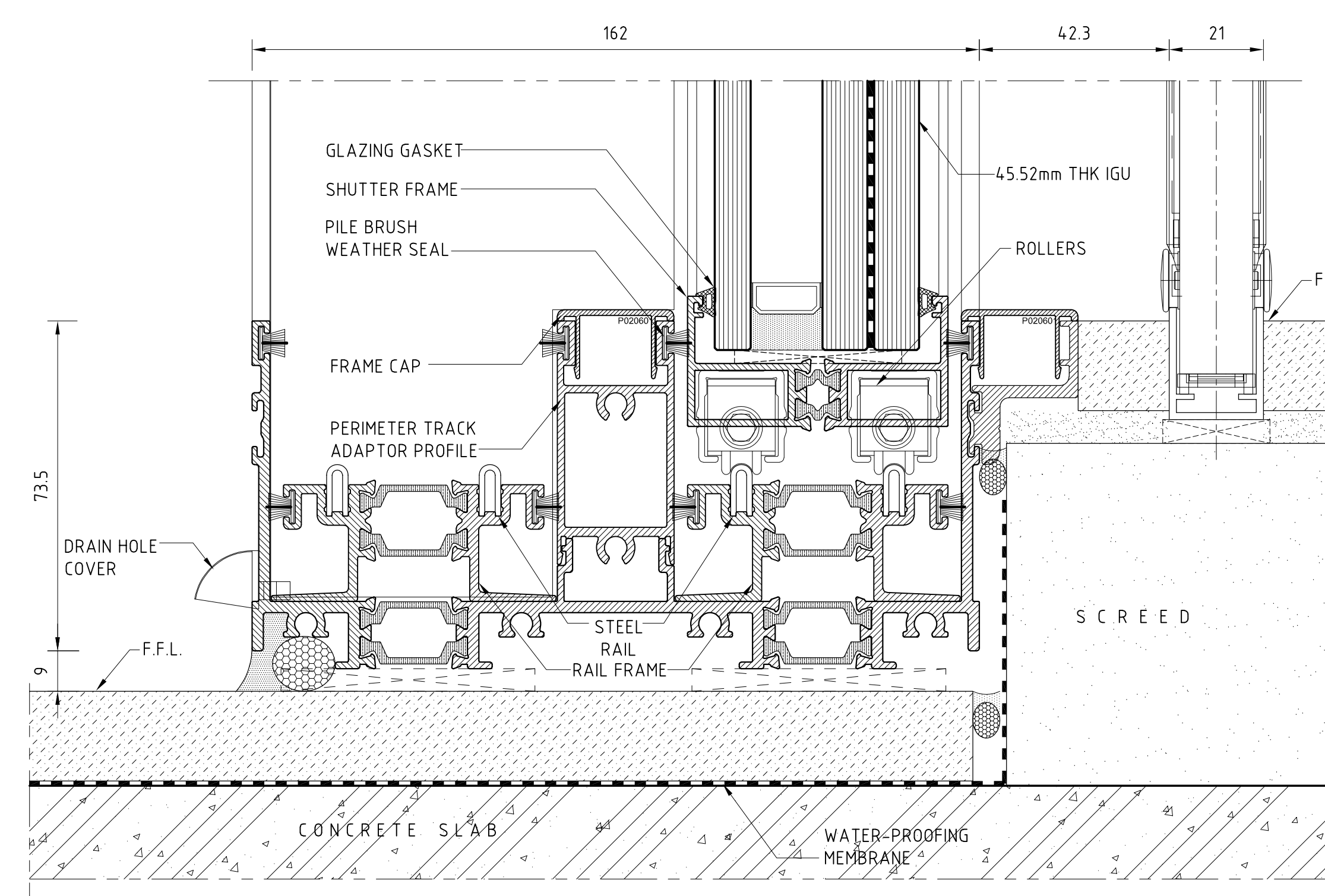
BOTTOM RAIL DETAIL
